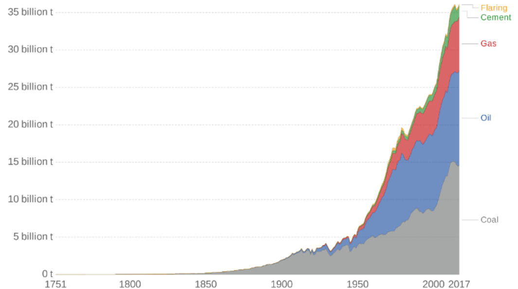
CO 2 emissions by fuel type, World
